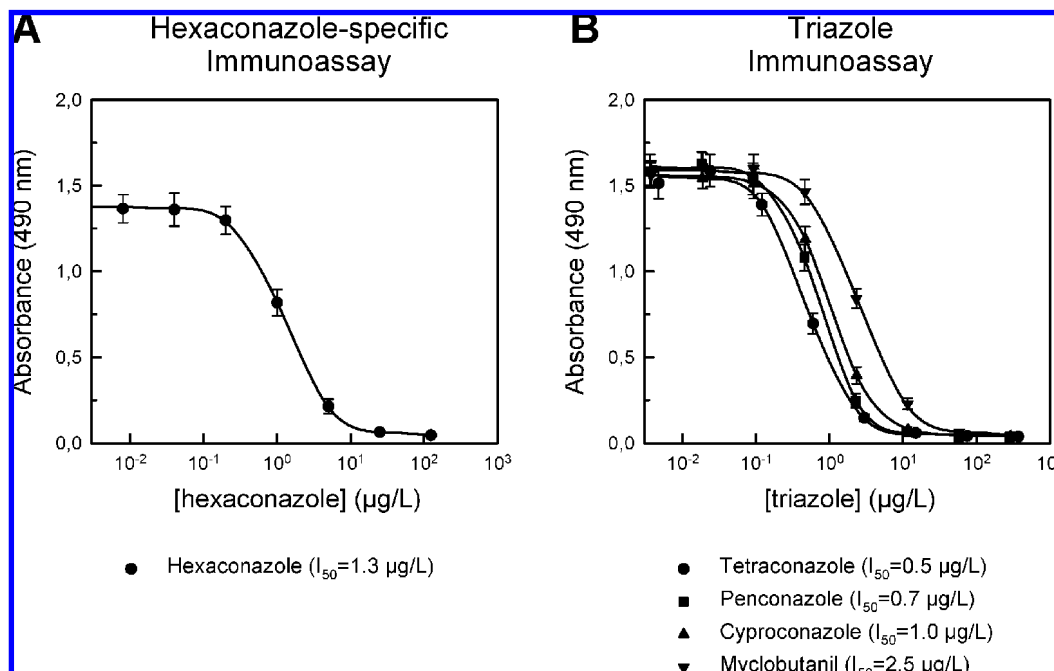
Figure 4. (A) Representative standard curve for hexaconazole obtained under optimized conditions: assay hapten, OVA–DTPH (2 \mu\text{g}/\text{mL} ) and HH-14 mAb (60 ng/mL); assay buffer, PBS containing 0.0025% Tween 20 and 0.25% DMF. (B) Representative standard curve for detected triazoles: assay hapten, OVA–HH (1 \mu\text{g}/\text{mL} ) and DTPH-41 mAb (30 ng/mL); the same assay buffer as above. Each point represents the mean value \pm standard deviation (SD) of three replicates.
