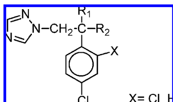
Figure 1. Common structure to several triazole fungicides: bromuconazole, cyproconazole, hexaconazole, myclobutanil, penconazole, propiconazole, and tetraconazole.
